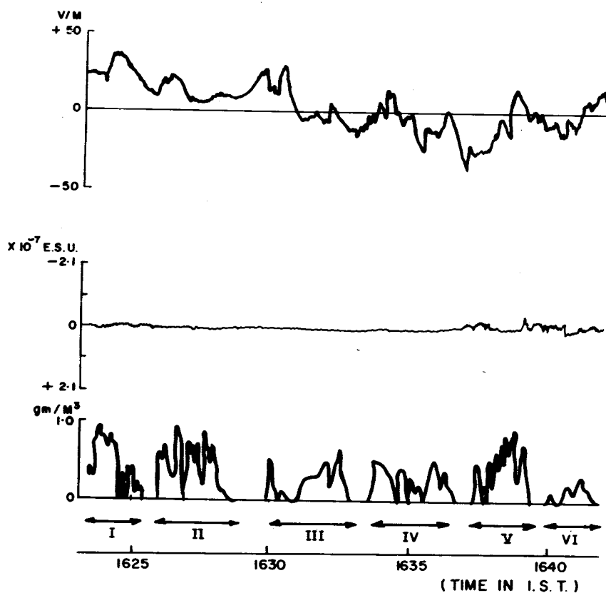
FIG. 2. Variations of potential gradient, cloud droplet charge and liquid water content during cloud traverses I-VI case 3, dissipation, at Bombay on 24 September 1974.
